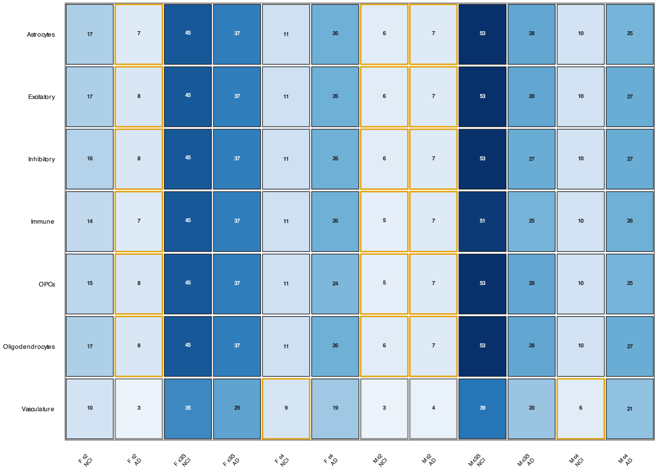
Donors passing the 20-nucleus threshold
