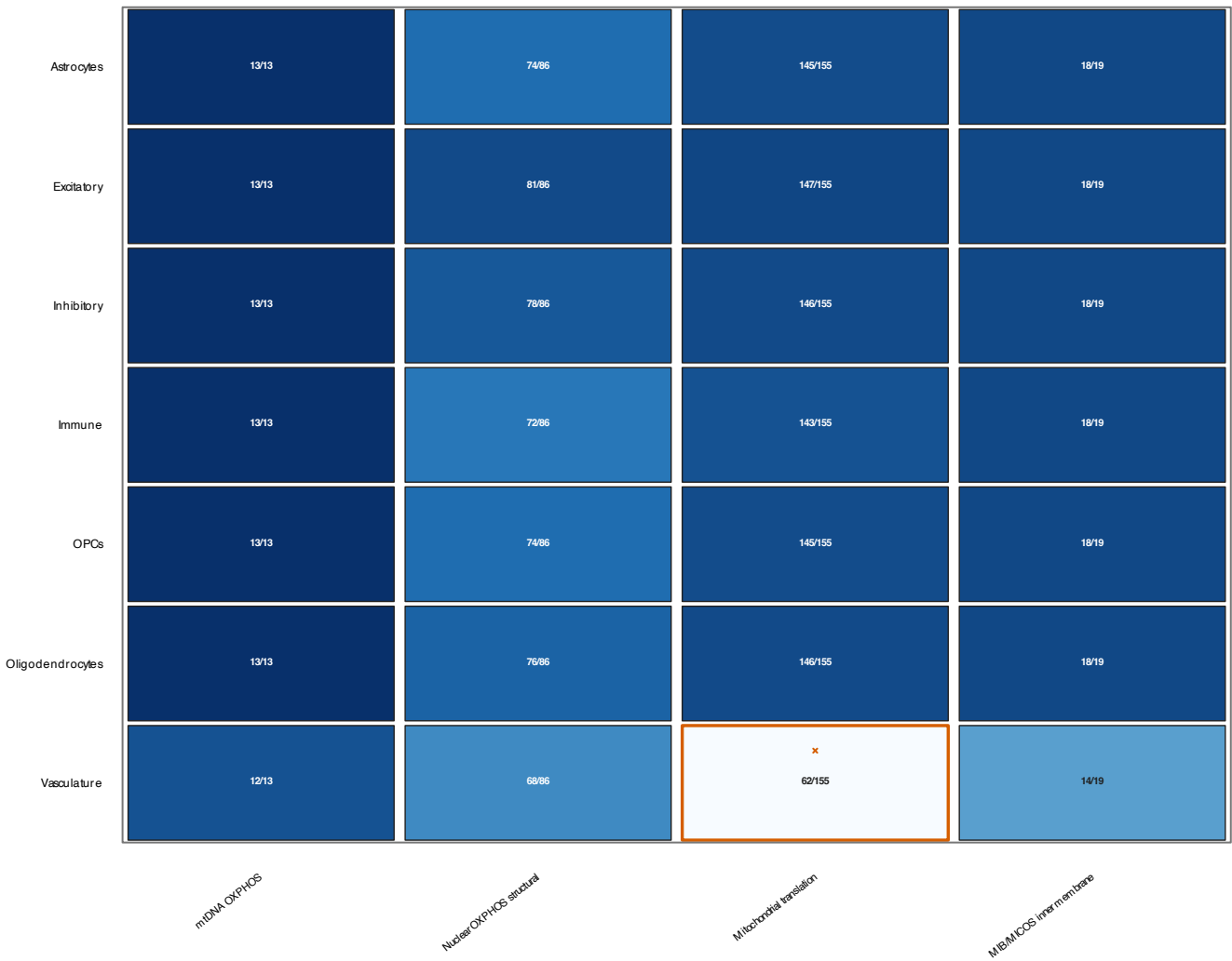
Admitted/reference module genes
